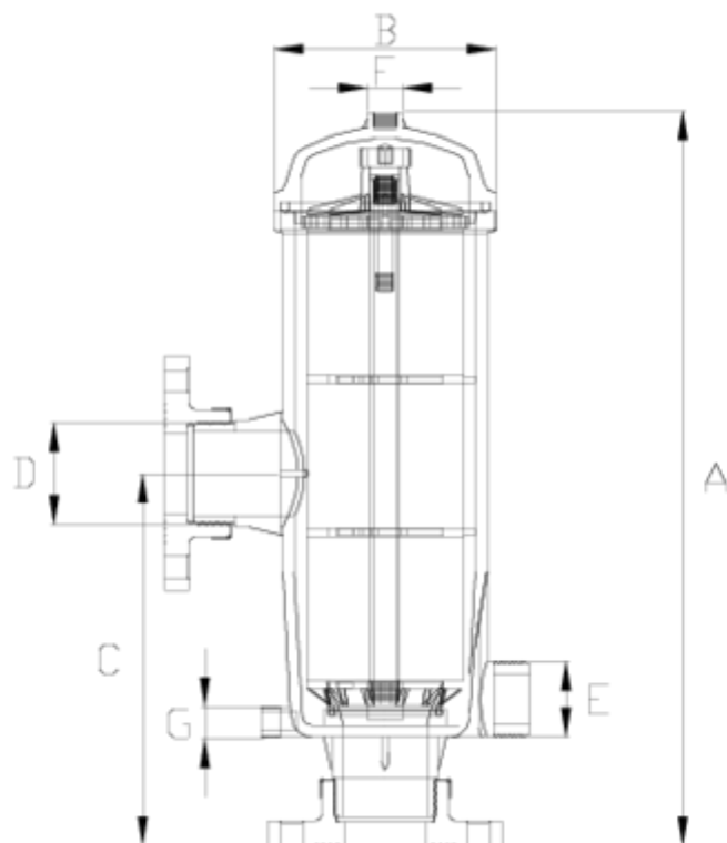
ITEM 319 | Outler with flanges
