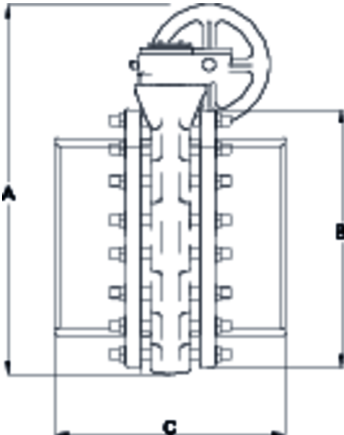
ITEM 187XL | Implex butterfly valve flanges with manual reductor 355
