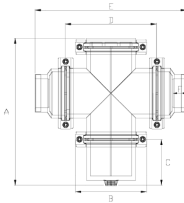
ITEM 523 | Female threaded outlet - Strainer
