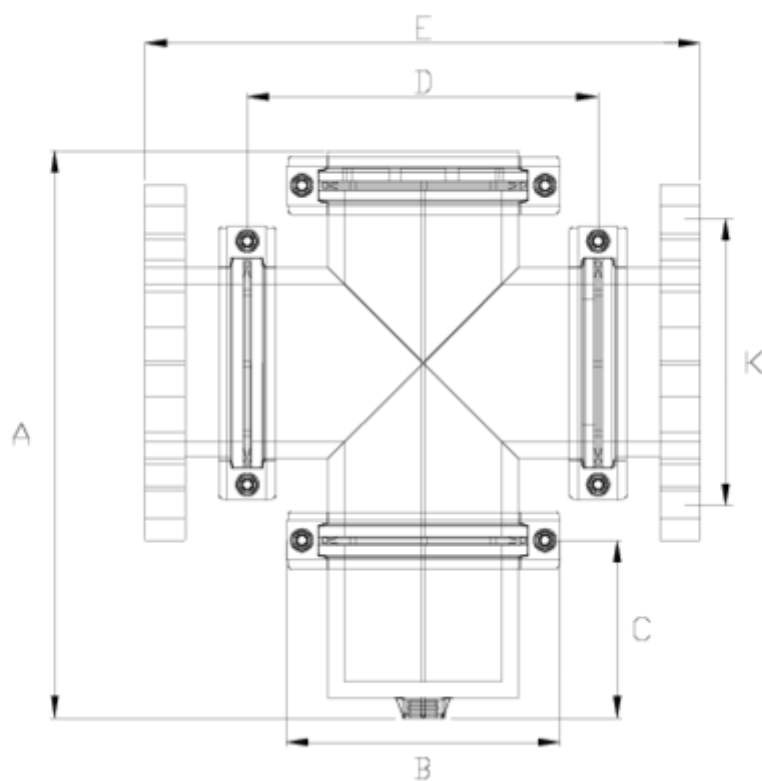
ITEM 524 | Flange outlet - Strainer
