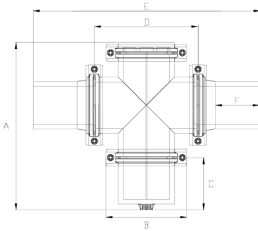
ITEM 522 | PE-PE outlet - Strainer
