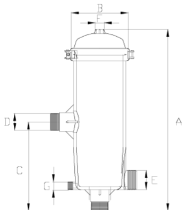
ITEM 318 | Threaded outlet "BSP" super
